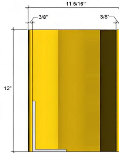
CRESCENT - DETAIL
