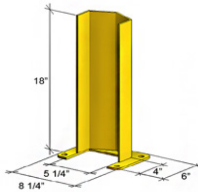
ITEM # RP18 18" RACK POST PROTECTOR
