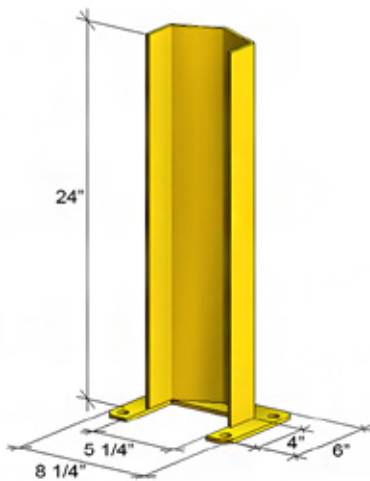
ITEM # RP24 24" RACK POST (PROTECTOR)
